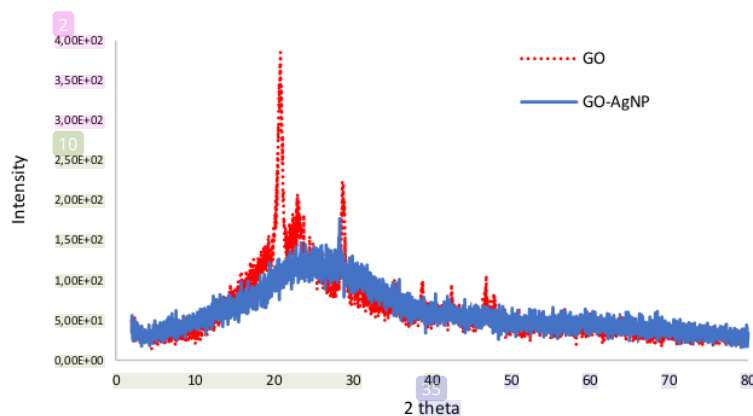
Figure 8. Diffractogram results of GO (dashed-red line) and GO-AgNP (solid-blue line) samples.
