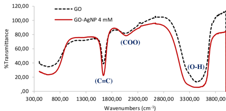
Figure 9. FTIR results for GO and GO-AgNP samples.
