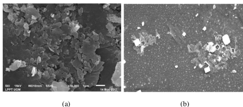
Figure 5. SEM-EDX images with 10,000X magnification for GO (a) and GO-AgNP mixture (b).
