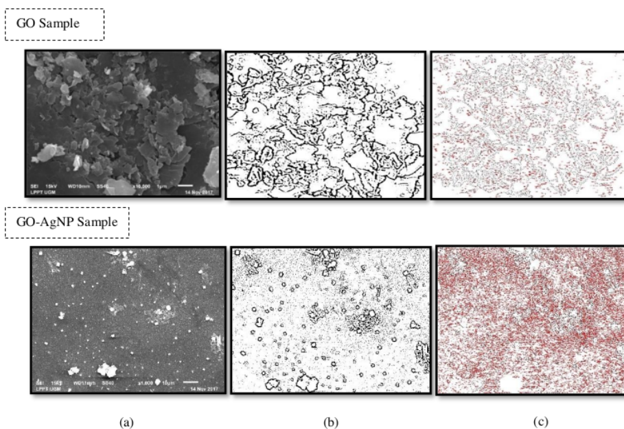
Figure 6. Results of SEM image processing using Image-J: (a) original sampling, (b) sample after threshold, and (c) sample outline image.
